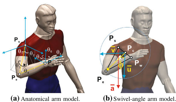
Fig. 2 Two kinematic models for the arm motion analysis [(rendered from Li et al. (2014)]
