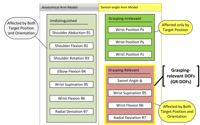
Fig. 3 Comparison between the two kinematic arm models
