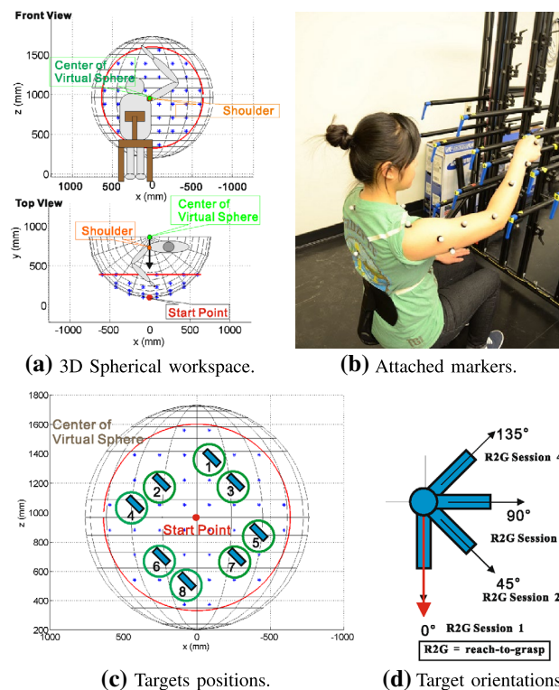
Fig. 1 Experimental setup: a the right shoulder of the participant is aligned with the center of the spherical workspace; b markers are attached to the right arm and the torso for position tracking; c eight targets are involved in the reach-to-grasp experiment; d in the four reach-to-grasp sessions, the handles are oriented at 0°, 45°, 90°, 135° in the plane faced by the participant, with respect to the direction of gravity
