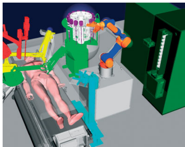
Figure 12. Primitives-based obstacle model
