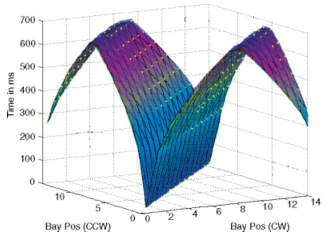
Figure 9. Movement time measured between each possible pair of tool positions during multiple tests ( n = 1350 ). Worst case movement time was 648 \pm 8 ms
