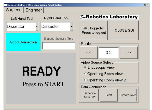
Fig. 3. SGUI window
