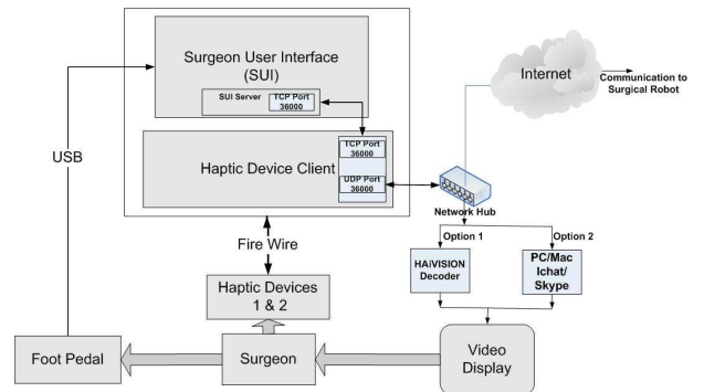
Fig. 2. Surgeon site software block diagram
