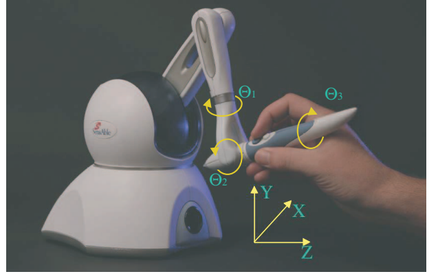
Fig. 5. Reference frame and orientation axes used in communication with surgical robot. (Image courtesy SensAble Technologies.)
