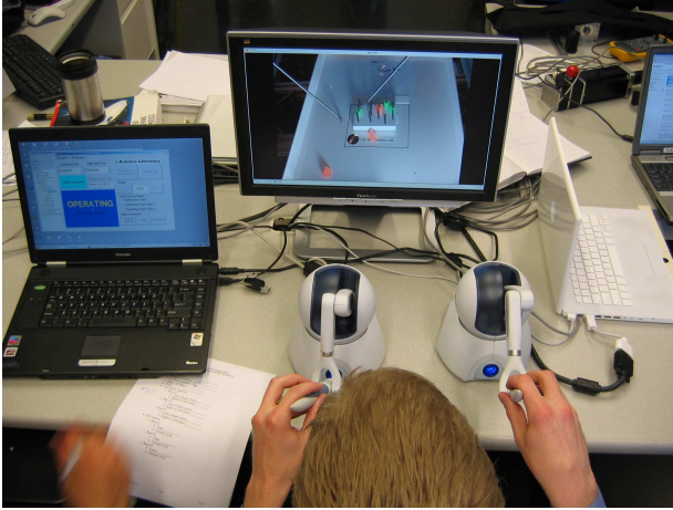
Fig. 4. System setup. SGUI (Fig. 3) appears on the laptop screen, surgical video transmission on the LCD monitor behind two Omni haptic devices. Setup is shown in-use during the NEEMO-12 experiment.
