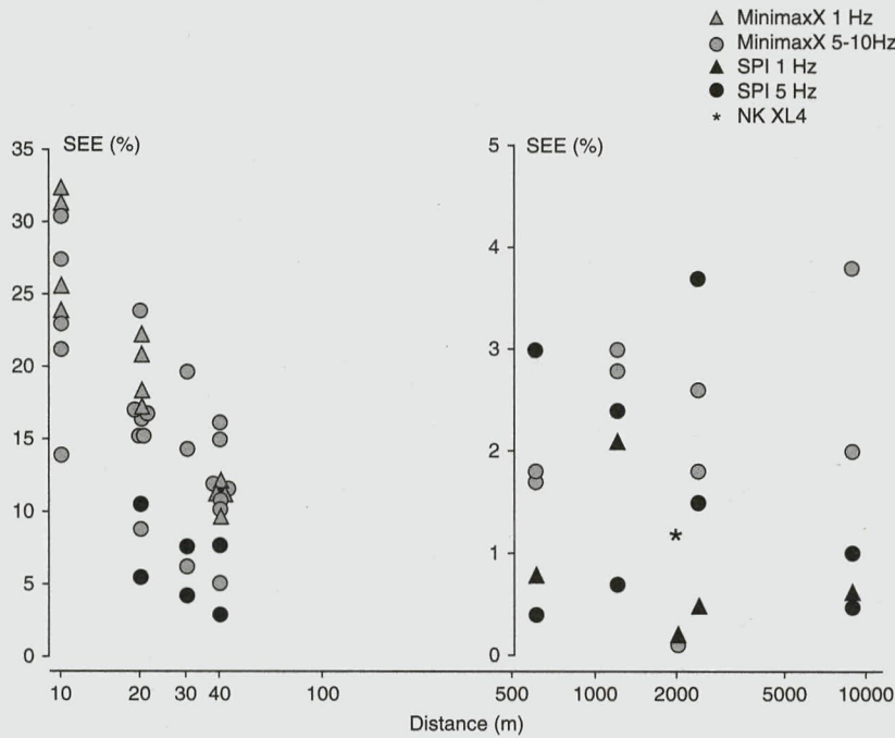
Fig. 1. Plot of the standard error of the estimate for each measurement device over various distances. NK = Nielsen Kellerman impeller; SEE = standard error of the estimate.
