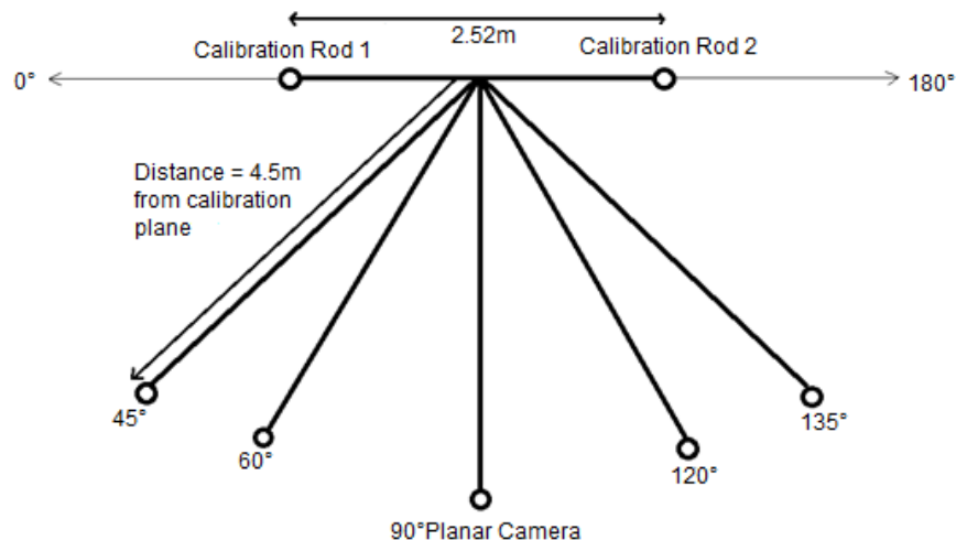
Figure 1: Diagram of testing setup as viewed from above.
