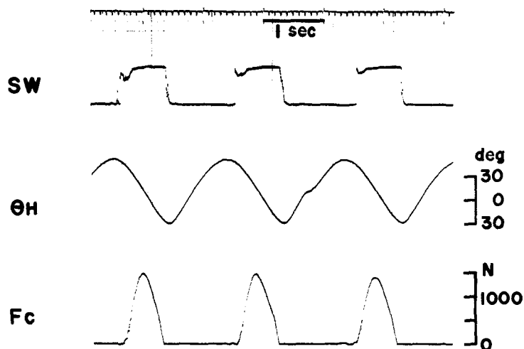
Fig. 2. A recording showing the time (SW) when the oar blade is in or out of water, the angular displacement of the oar ( \theta_H ), and the force applied to the pin ( F_C ) during a rowing stroke. \theta_H=0 represents the oar being perpendicular to the water flow
