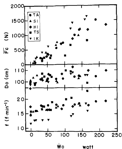
Fig. 3. Mean force applied to the oarlock pin, \bar{F}_C , displacement of handgrip, D_O , and stroke frequency, f , as functions of mechanical power, \dot{W}_O
